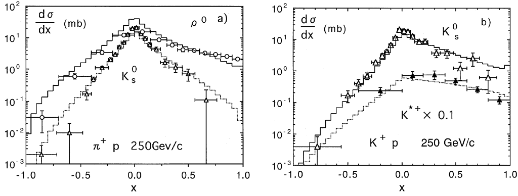
Fig. 5. Feynman x distributions of a \rho^0 and K_S^0 in \pi^+p and b K_S^0 and K^{*+} in K^+p collisions at p_L = 250 GeV/c. Experimental data are taken from [24]
