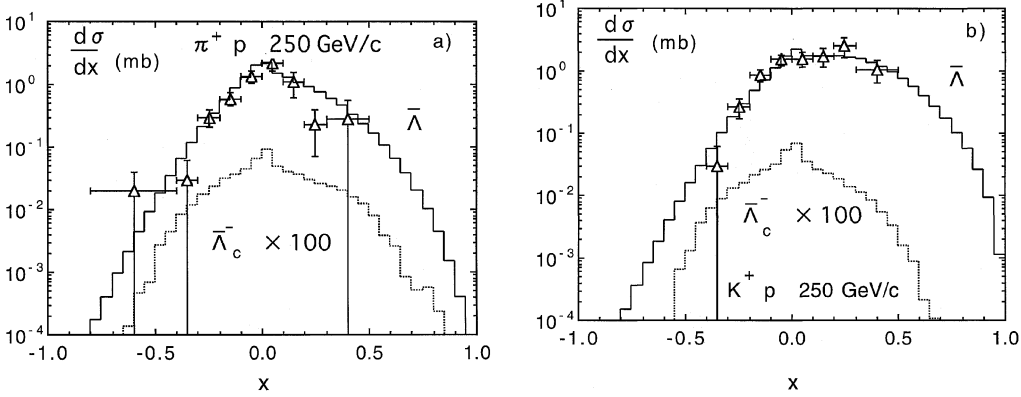
Fig. 9. Feynman x distributions of \bar{\Lambda} and \bar{\Lambda}_c in a \pi^+p and b K^+p collisions at p_L = 250 GeV/c. Experimental data are taken from [23]
