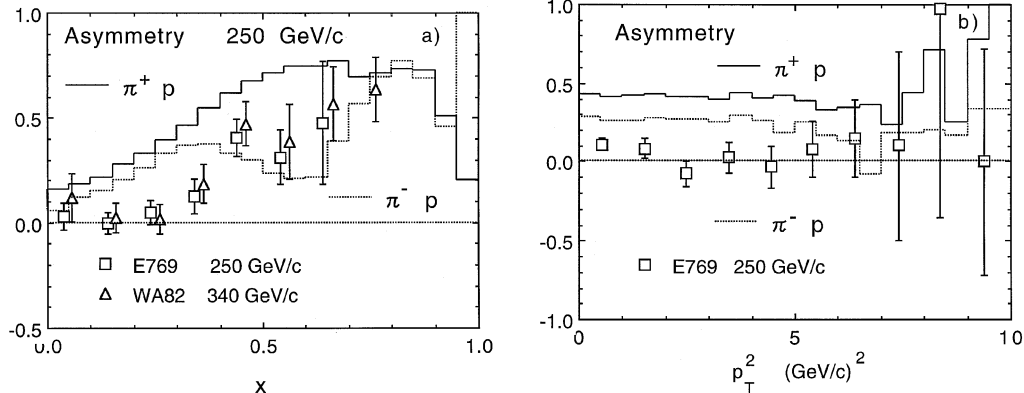
Fig. 7. Asymmetries of D^\pm in \pi^\pm p collisions: a vs. x and b vs. p_T^2 at 0.1 < x < 0.7 . Experimental data are taken from [1] and [2]
