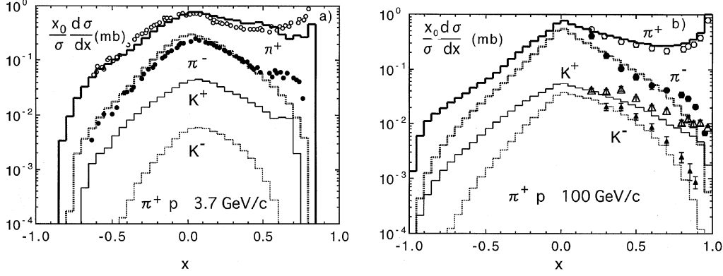
Fig. 3. Invariant x distributions of \pi^\pm and K^\pm in \pi^+p collisions at a p_L = 3.7 GeV/c and b p_L = 100 GeV/c. Experimental data are taken from [21] and [22]
