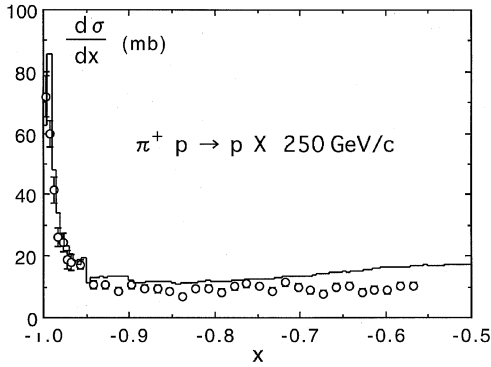
Fig. 4. Calculated values for x distributions of p in \pi^+p collisions at p_L = 250 GeV/c. Experimental data are taken from [23]
