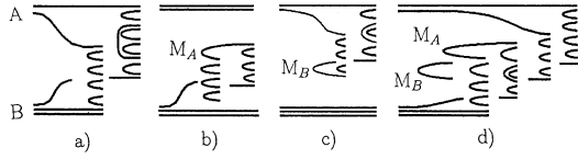
Fig. 1. The reaction mechanisms in AB collision: a Non-diffractive dissociation type, b,c Single-diffractive dissociation type and d double-diffractive dissociation type mechanisms
