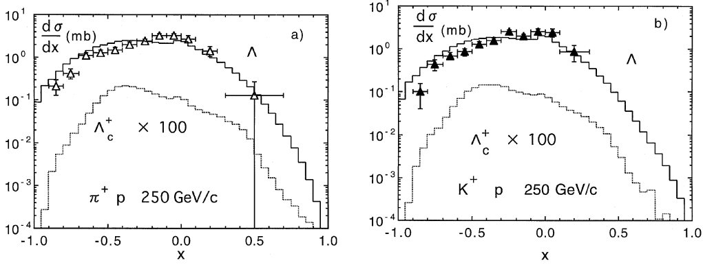
Fig. 8. Feynman x distributions of \Lambda and \Lambda_c in a \pi^+p and b K^+p collisions at p_L = 250 GeV/c. Experimental data are taken from [23]
