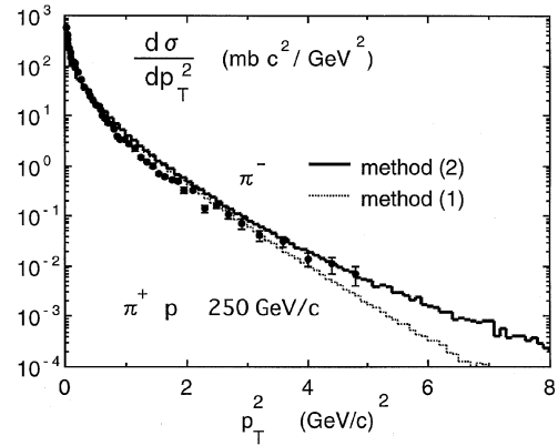
Fig. 2. Calculated values for p_T^2 distributions of \pi^- in \pi^+p collisions at p_L = 250 GeV/c. Experimental data are taken from [20]
